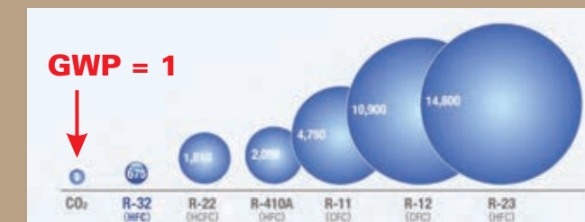
100 year global warming potential of different refrigerants
